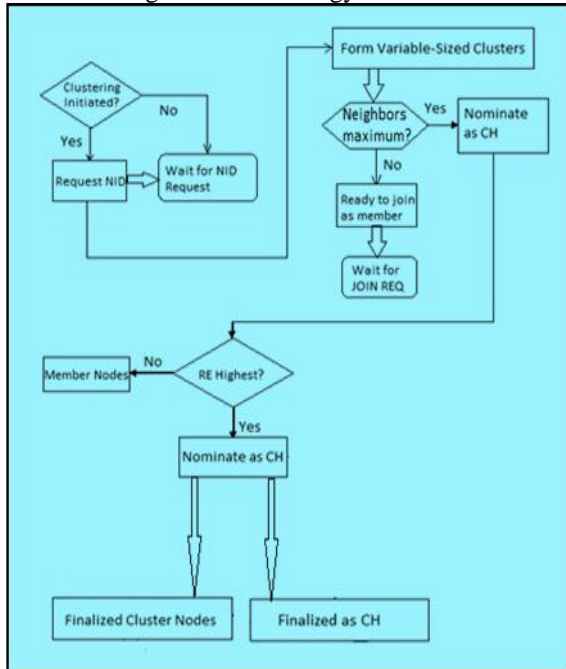
Figure 4: Mechanism of Cluster Head Selection in the Proposed Algorithm
