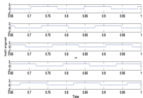
Fig 6 Hall Signal
