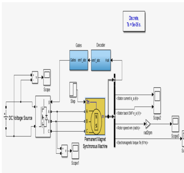
Fig4 Simulink model of three phase
