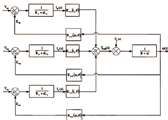
Fig 2 Model of a BLDC motor
