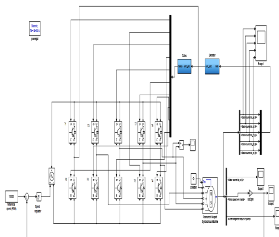
Fig 5 Simulink model of five phase
