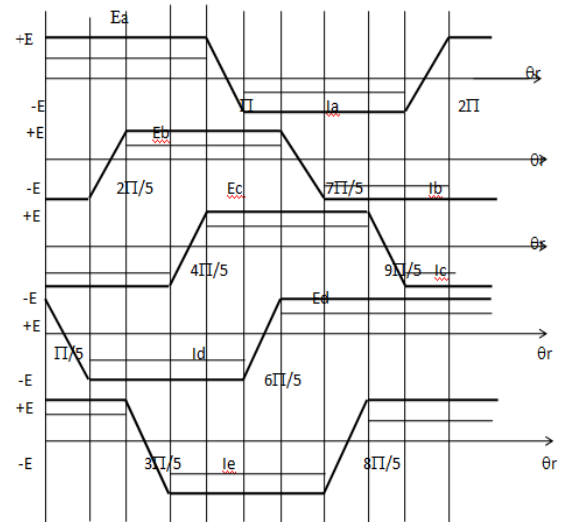
Fig 3 Trapezoidal waveform
